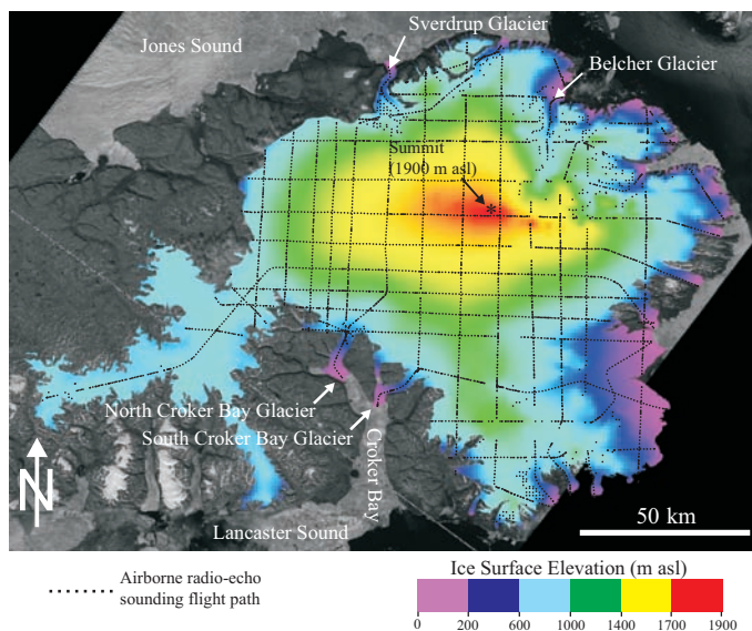
FIG. 2. Most recent ice surface elevation model of the Devon Island ice cap. This digital elevation model (DEM) is derived from airborne radar surveys completed in 2000 (from Dowdeswell et al., 2004).
