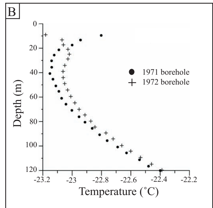
FIG. 5. Englacial temperature profiles: (A) in the top 14 m of the Sverdrup Glacier (from Keeler, 1964) and (B) in the top 120 m of a summit borehole (from Paterson and Clarke, 1978).
