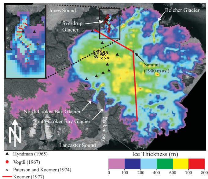
FIG. 3. Ice thickness distribution across the Devon Island ice cap from airborne radar surveys completed in 2000 (from Dowdeswell et al., 2004) and locations of previous ice thickness surveys (from Hyndman, 1965; Vogtli, 1967; Paterson and Koerner, 1974; Koerner, 1977a).
