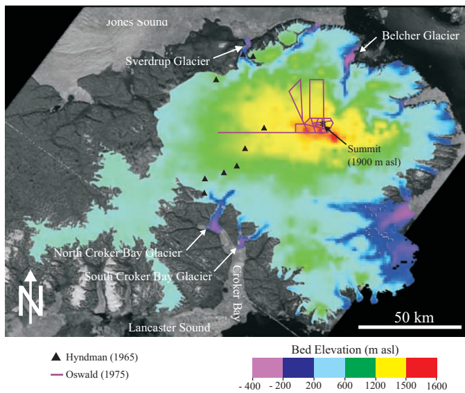
FIG. 4. Bed elevation DEM of the Devon Island ice cap derived from airborne radar surveys completed in 2000 (from Dowdeswell et al., 2004) and locations of previous bed condition measurements (from Oswald, 1975; Hyndman, 1965).
