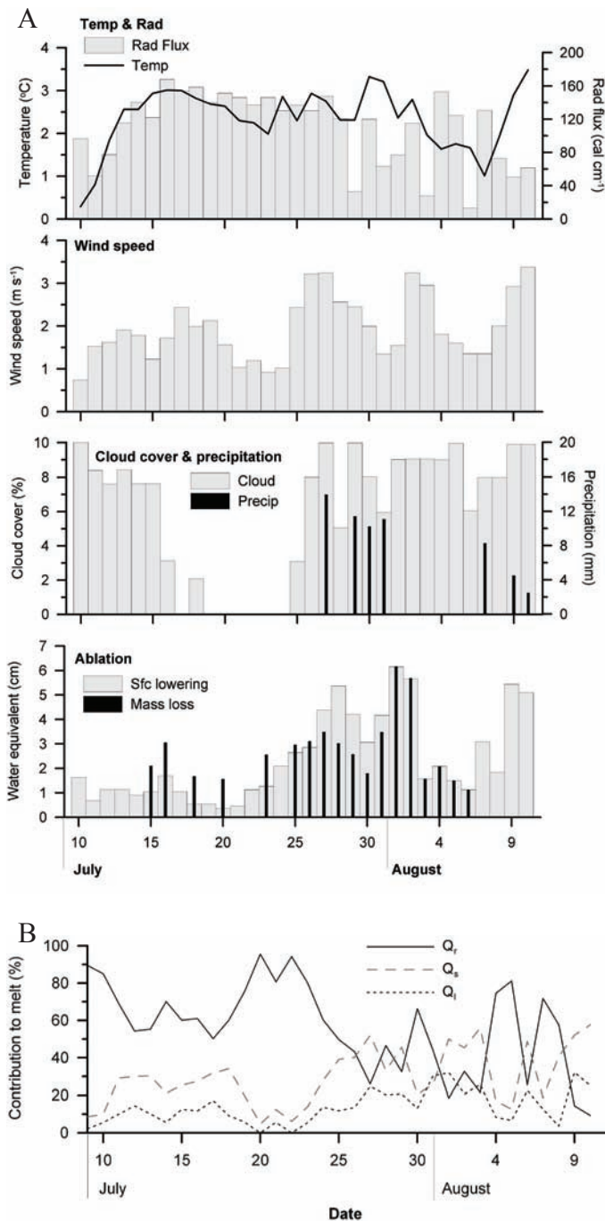
FIG. 6. Measurements from the Sverdrup Glacier, summer 1963: (A) net radiation and air temperature, wind speed, cloud cover and precipitation, mass loss, and surface lowering; and, (B) declining contribution of net radiation ( Q_r ) to melt over time, compared to sensible ( Q_s ) and latent ( Q_l ) fluxes (Keeler, 1964). Note that mass loss was measured from core samples of the surface weathering rind, while surface lowering ablation was calculated from ablation stake measurements multiplied by a constant density value.
