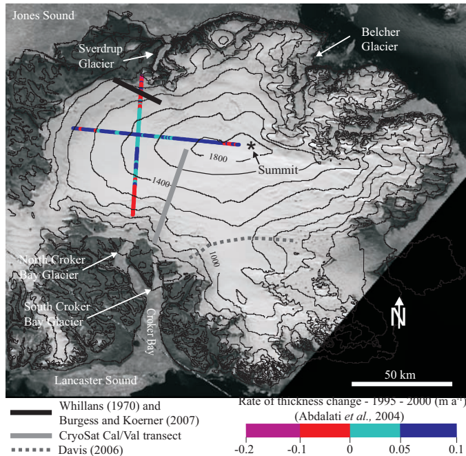
FIG. 9. Surface elevation change across the Devon Island ice cap derived from altimetry data (from Abdalati, 2004) and locations of field and remote sensing measurement transects from which changes in glacier surface elevation can be calculated.
