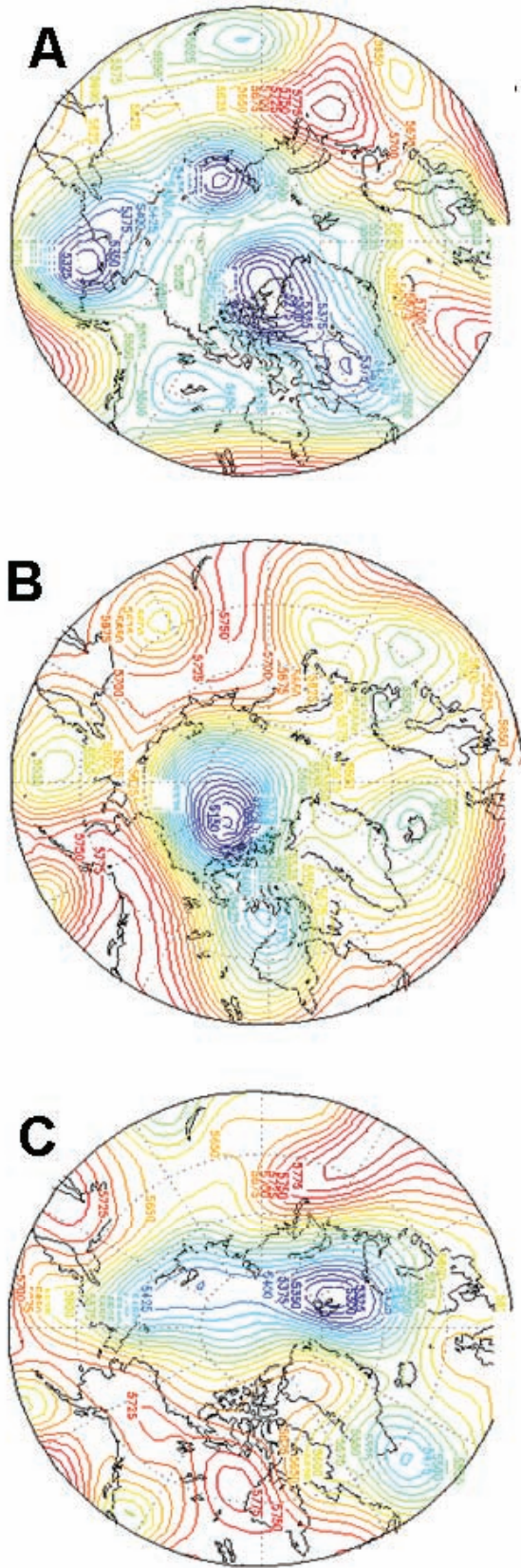
FIG. 7. 500 mb polar synoptic conditions observed to drive ice cap mass balance during 1961–74: (A) Type Ia, 27 June 1963; (B) Type IIa, 30 July 1962; and (C) Type IIIa, 17 July 1962 (from Alt, 1978). Images provided by the NOAA/ESRL Physical Sciences Division, Boulder, Colorado from http://www.cdc.noaa.gov/ . Contours show 500 mbar geopotential heights.
