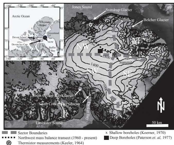
FIG. 1. Location of the Devon Island ice cap in the Canadian Arctic. NOW = North Open Water polynya. Contour lines are in meters above mean sea level. Mass balance sectors are labeled (from Mair et al., 2005). Locations of field-based mass balance measurement transects, ice core boreholes, shallow cores in the superimposed ice zone, and englacial thermistor string measurements are shown (from Keeler, 1964; Koerner, 1970a, b; Paterson et al., 1977).
