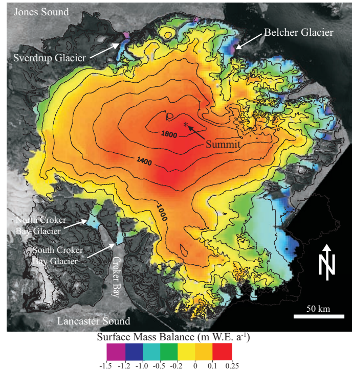
FIG. 11. Spatial pattern of mass balance across the Devon Island ice cap derived from field measurements and numerical modeling (from Mair et al., 2005).
