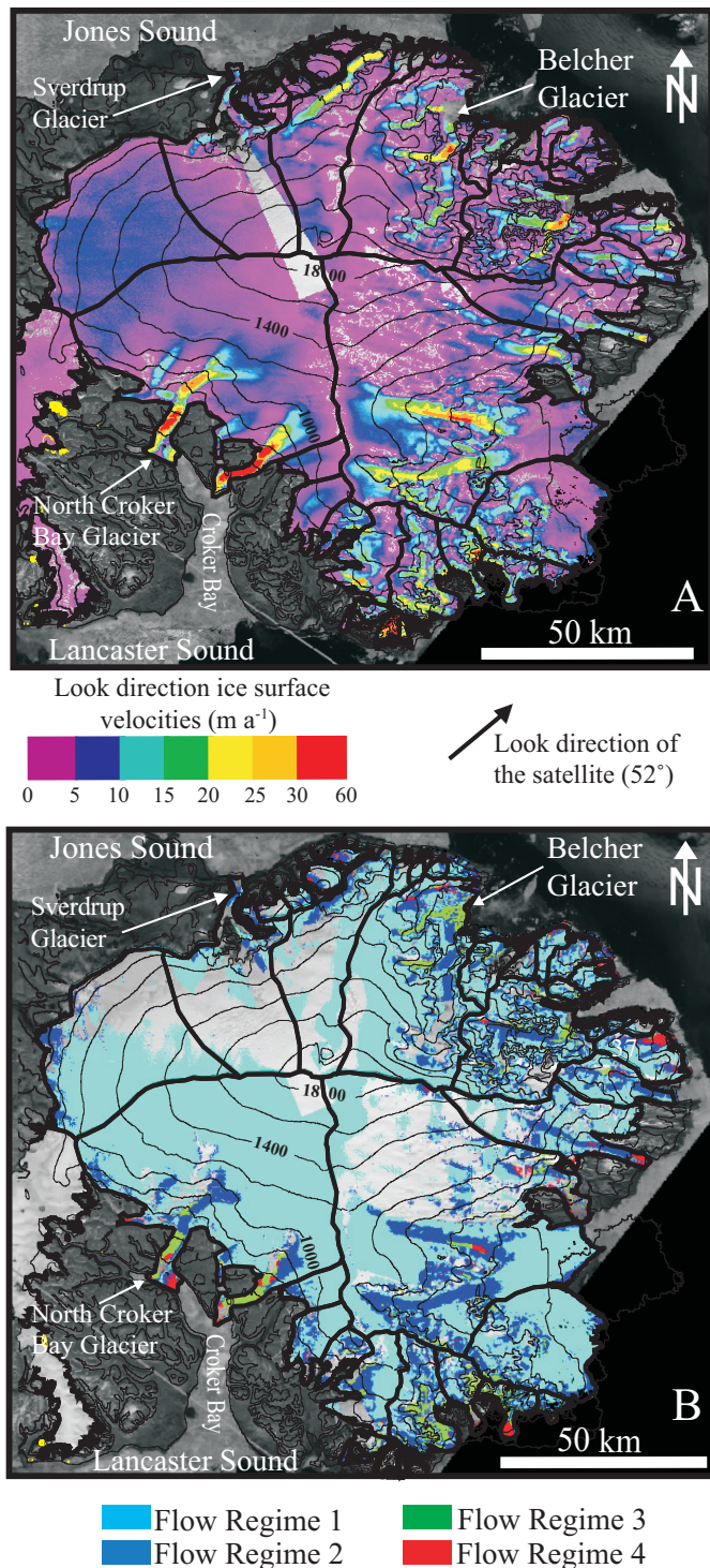
FIG. 8. (A) SAR-derived ice flow velocities across the Devon Island ice cap; and (B) distribution of four flow regime classes derived from surface velocity, ice thickness, and driving stress (from Burgess et al., 2005).
